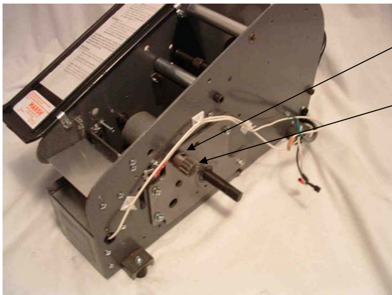
Fig 22 Gearbox/Motor Mount
