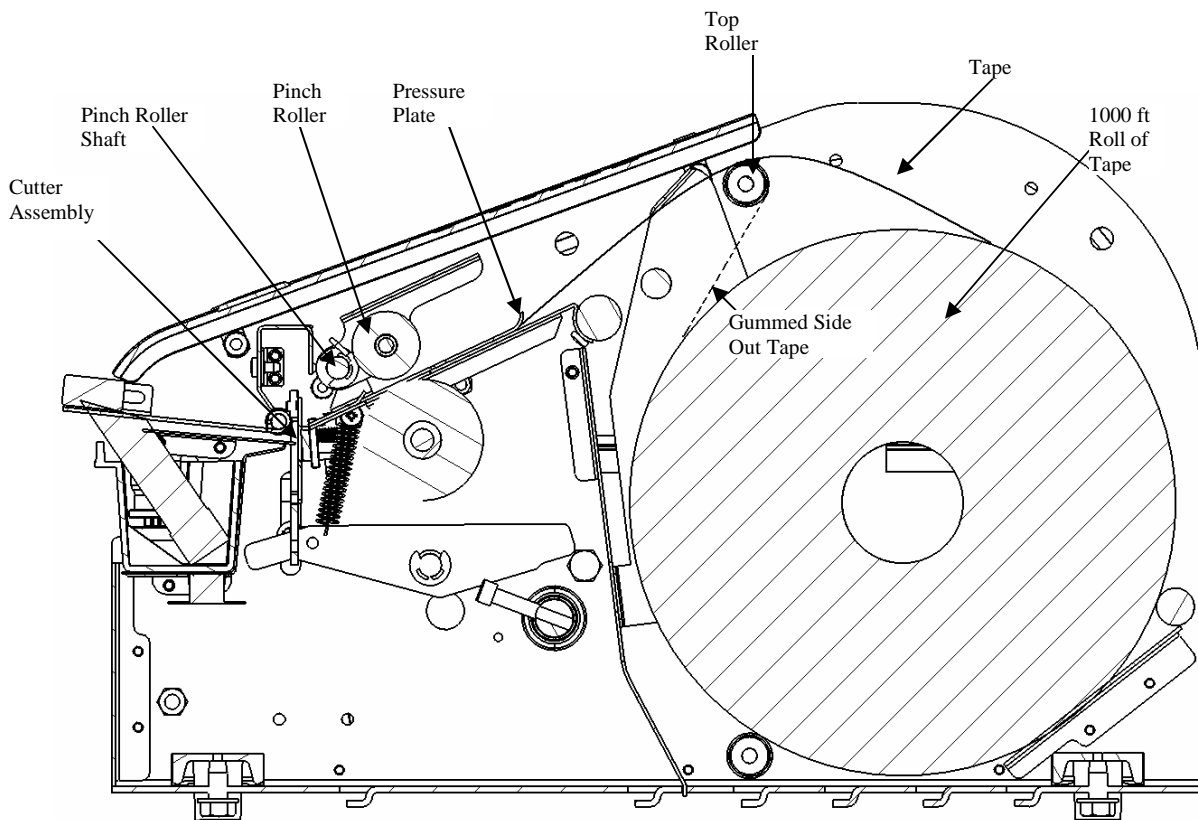
Figure 3 – Tape Routing
